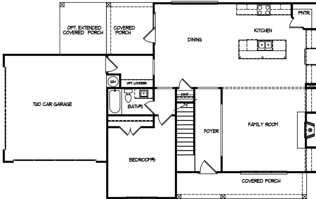
Main Level
