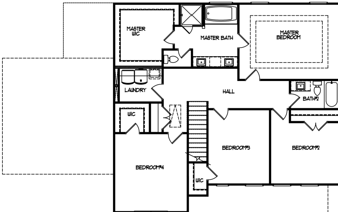
Upper Level
