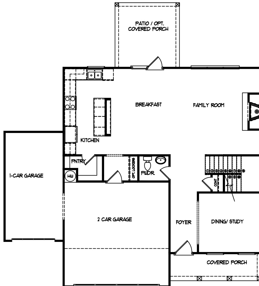
Main Level w/ 3rd Car Garage Opt.
